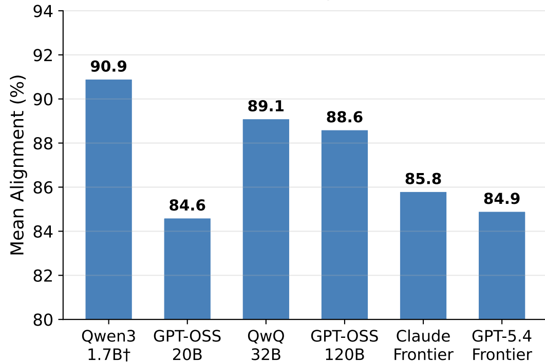
With GT
