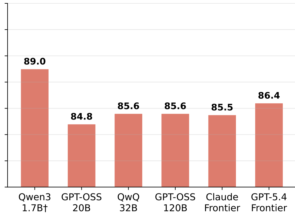
Without GT
